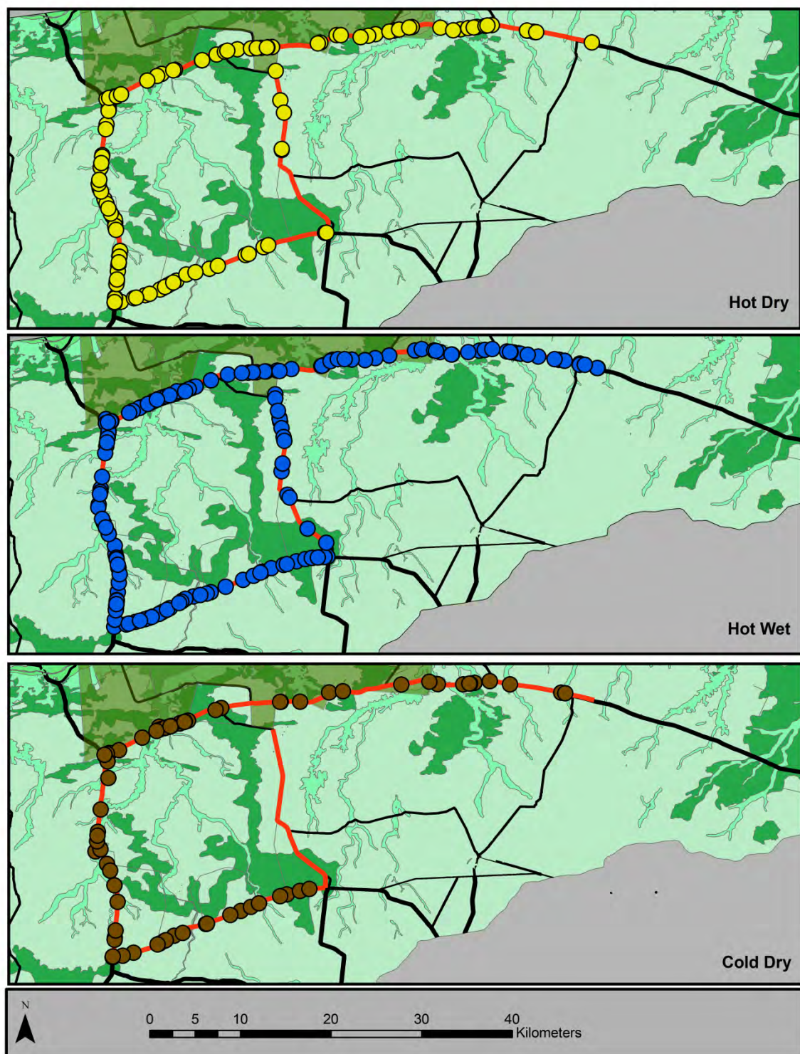
Figure 3: Three vegetation maps illustrating the location on the transects (100 km paved road and 20 km unpaved road) of Aves roadkill detected during the (a) hot/dry, (b) the hot/wet and (c) the cold/dry seasons in the GMTCA, South Africa. GIS data source: GeoNetwork (2000); Peace Parks Foundation (2010). (ArcGIS 9.3; map units: decimal degrees; not projected).
