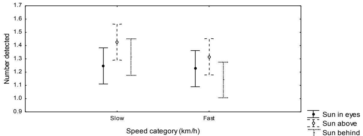
Figure 3.9 The difference between the position of the sun and the mean ( \pm 95% CI) number of large and small (see text 2.2.1) artificial roadkill detected at two pooled speeds (slow: 20-50 km.h -1 / fast: 60-100 km.h -1 ) during experimental testing along a 1 km section of paved road in the GMTFCA, South Africa.
